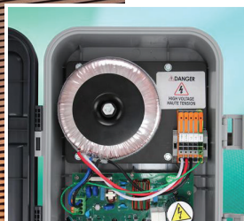
MV00540 Optional 480/600V Input Voltage Transformer Kit
