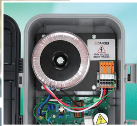
High Voltage Transformer Kit
