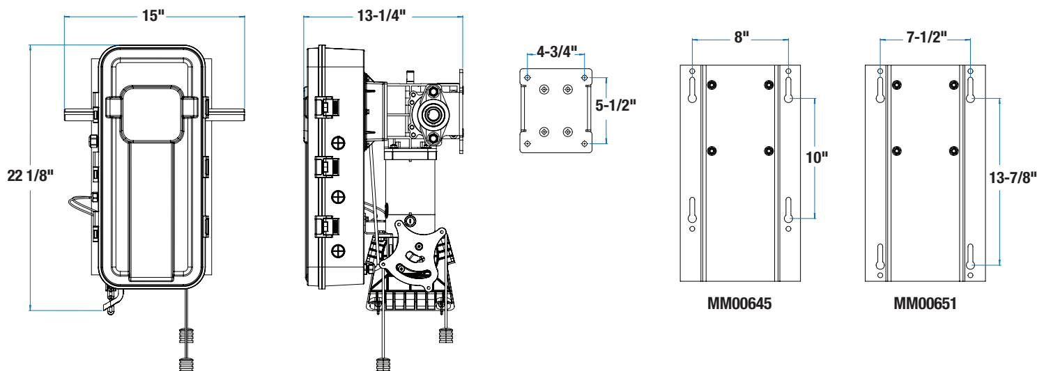
MV00541 Electromechanical Brake Kit
