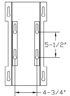
BRACKET MOUNT
