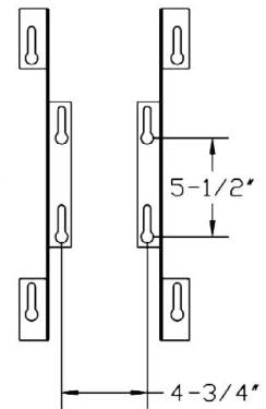
BRACKET MOUNT
