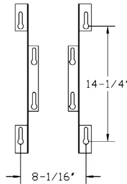
WALL MOUNT
